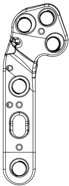
3.0 mm VAR-3130MPL-R
